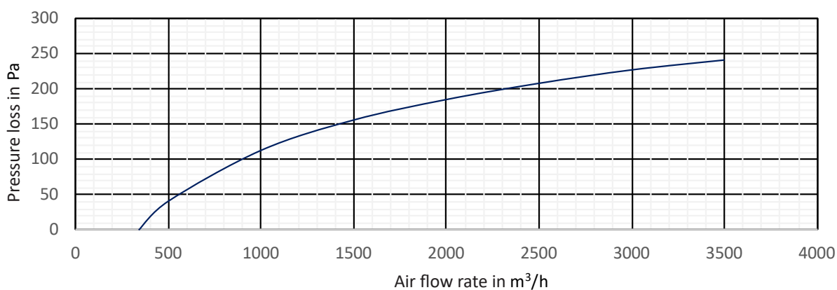
F7 pressure loss diagram for sizes 315, 355 and 400
