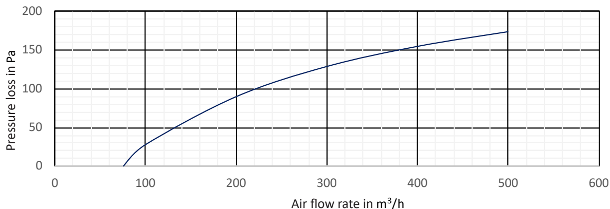
F7 pressure loss diagram for sizes 100, 125 and 160
