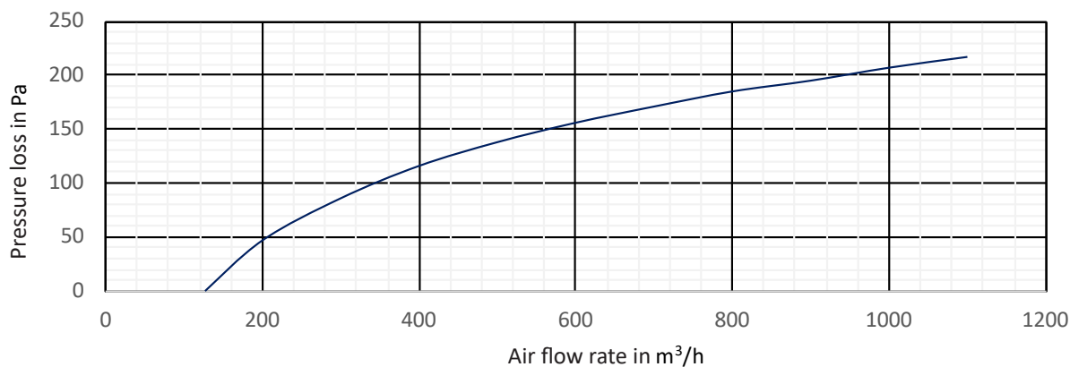
F7 pressure loss diagram for sizes 200 and 250
