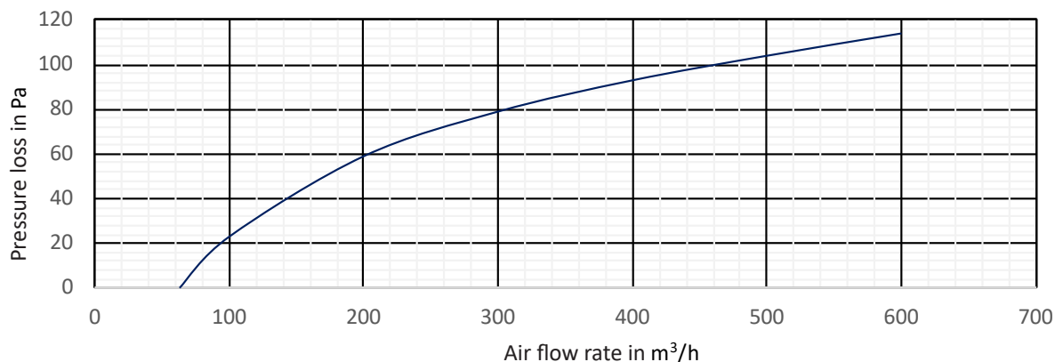
G4 pressure loss diagram for sizes 100, 125 and 160
