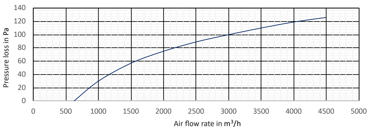
G4 pressure loss diagram for sizes 315, 355 and 400
