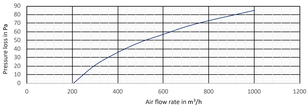
G4 pressure loss diagram for sizes 200 and 250
